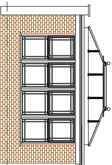
SIDE ELEVATION
